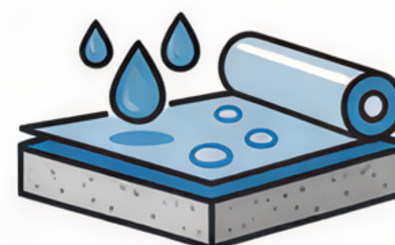
Moisture-prone concrete: use sealant or 6 mil polyethylene vapor barrier
